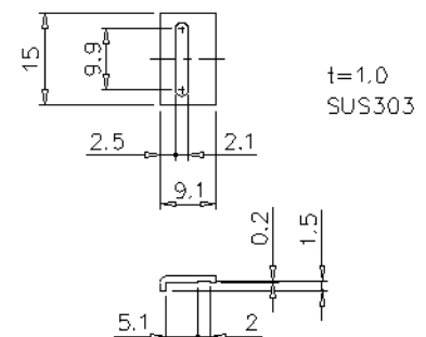
Mounting bracket
